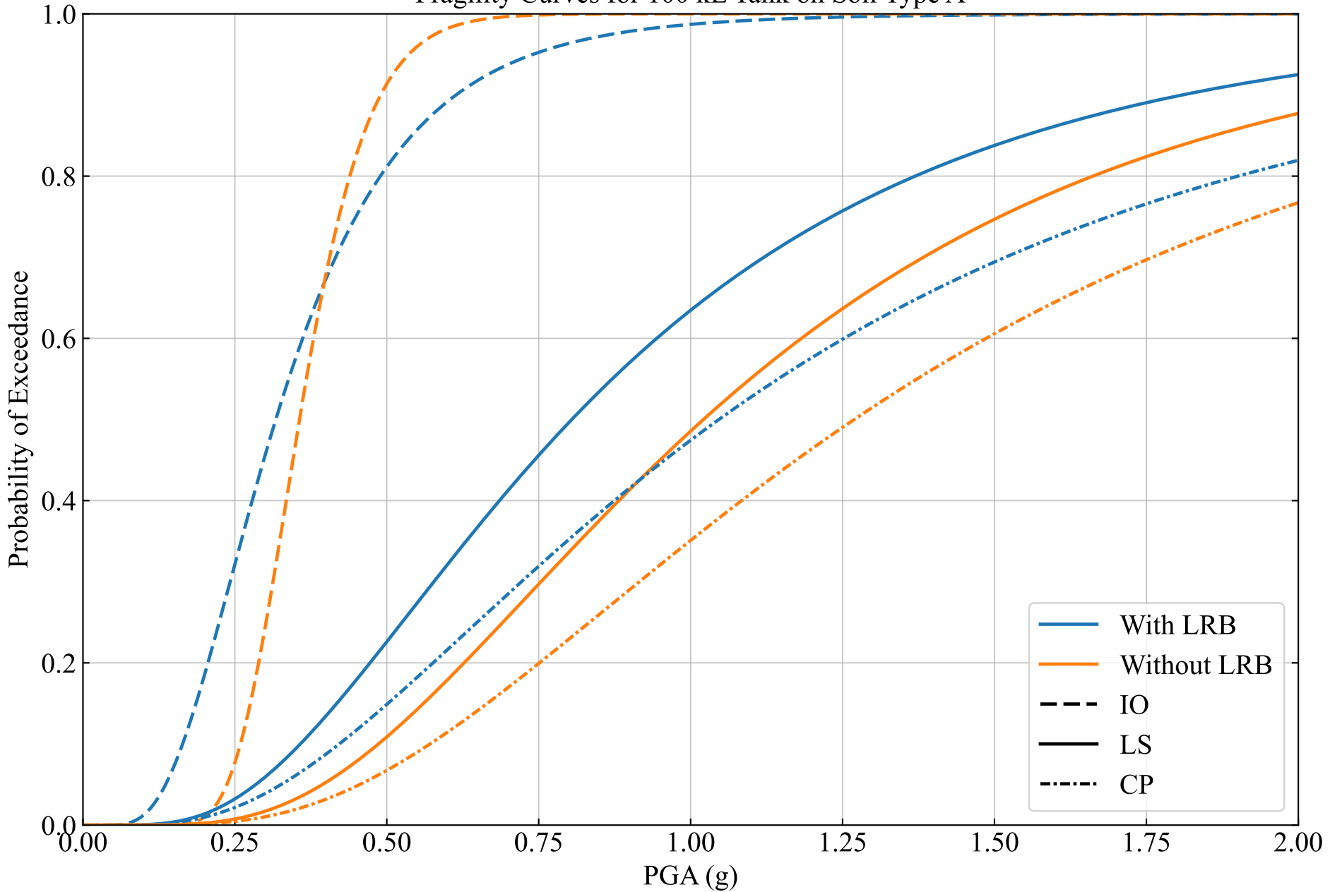
Fragility Curves for 100 kL Tank on Soil Type A
